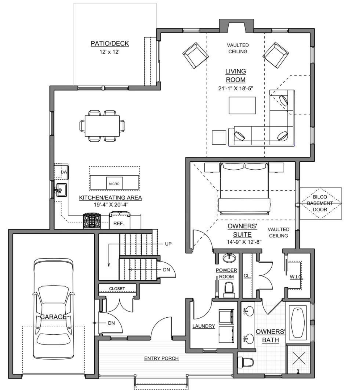
FIRST FLOOR PLAN - 1,497 G.S.F.
