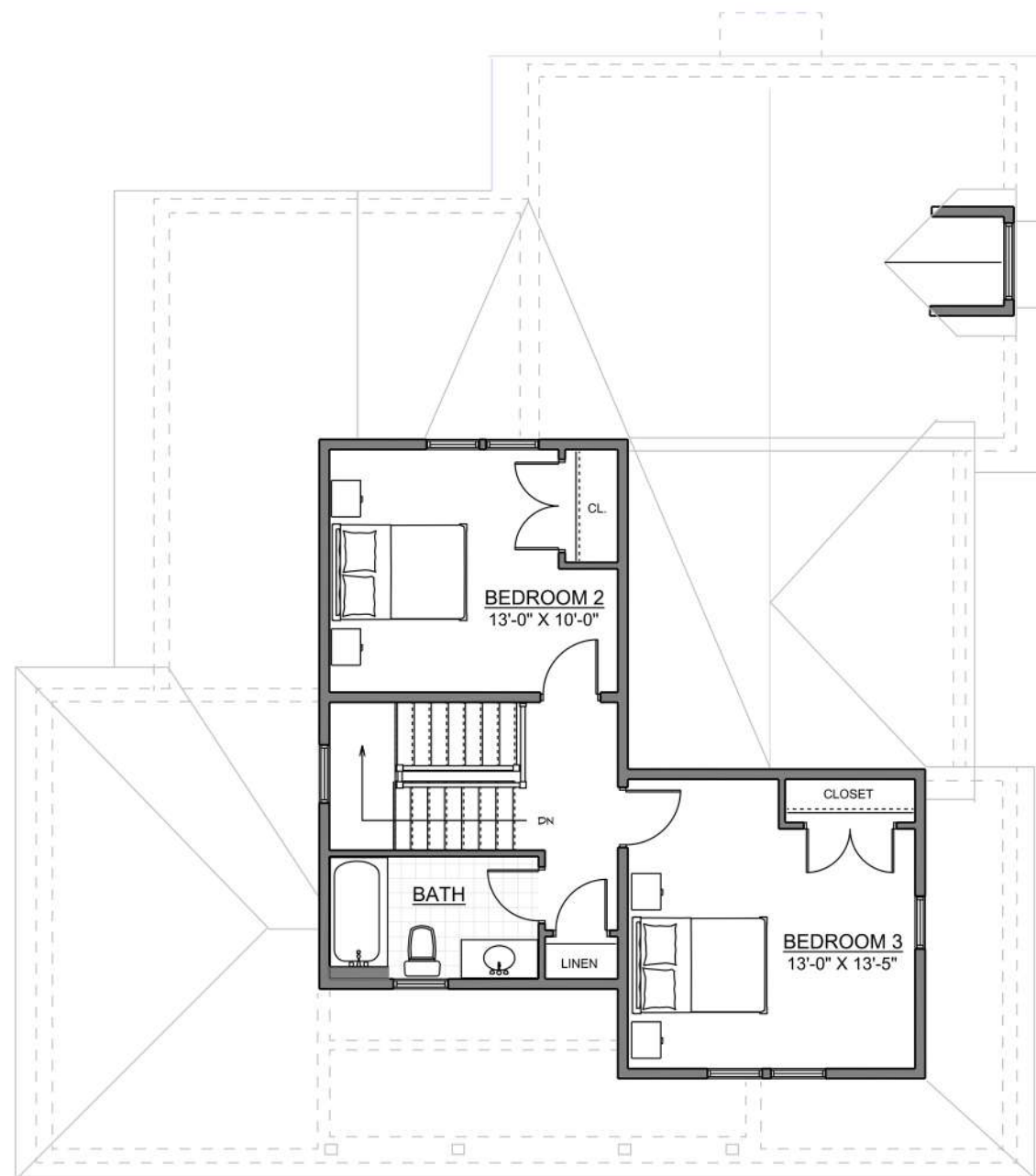
SECOND FLOOR PLAN - 463 G.S.F.
