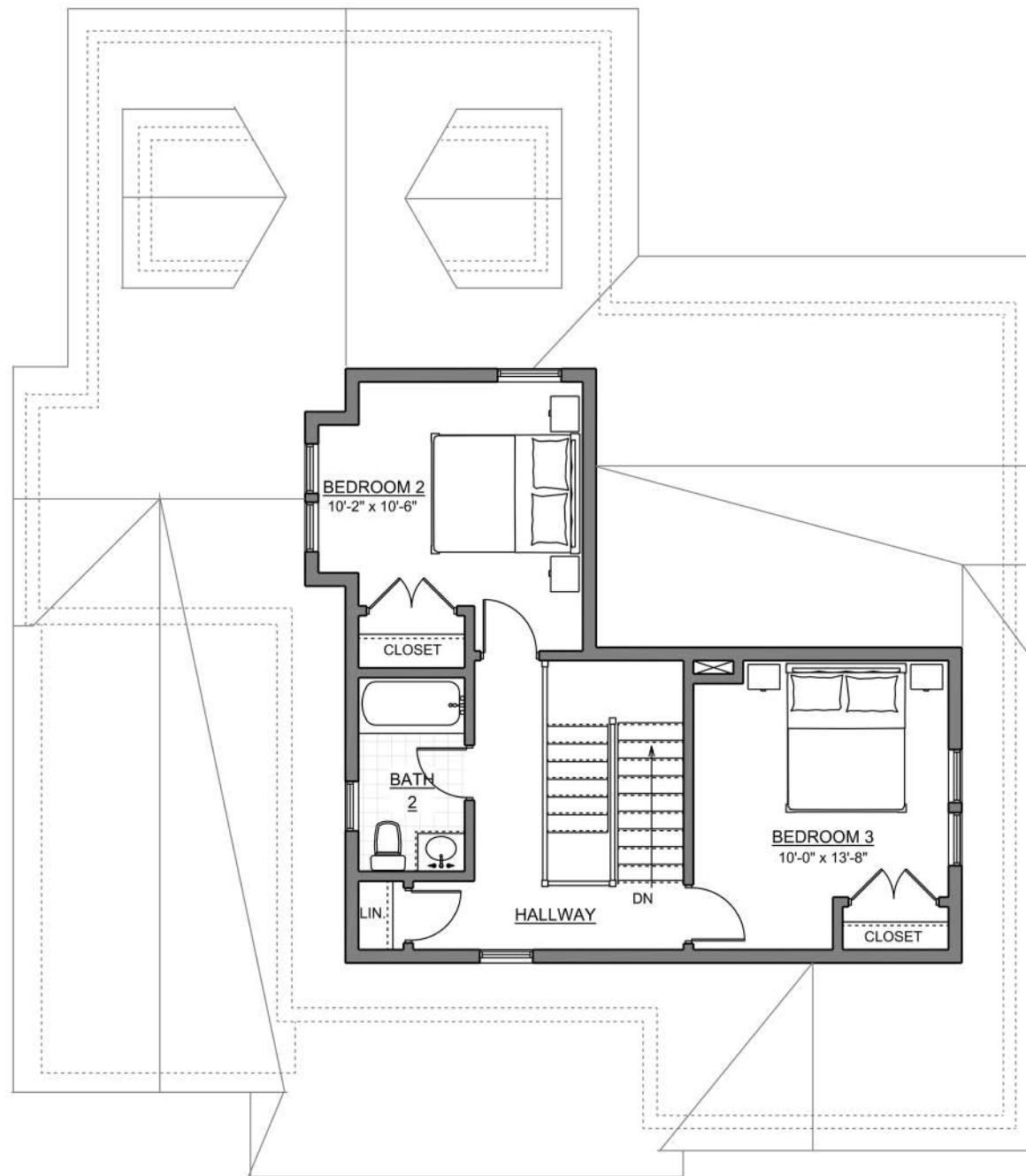
SECOND FLOOR PLAN - 509 G.S.F.
