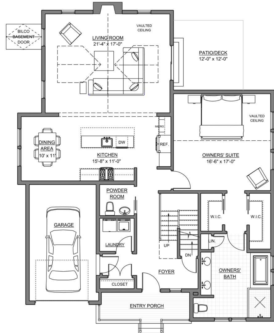
FIRST FLOOR PLAN - 1,620 G.S.F.
