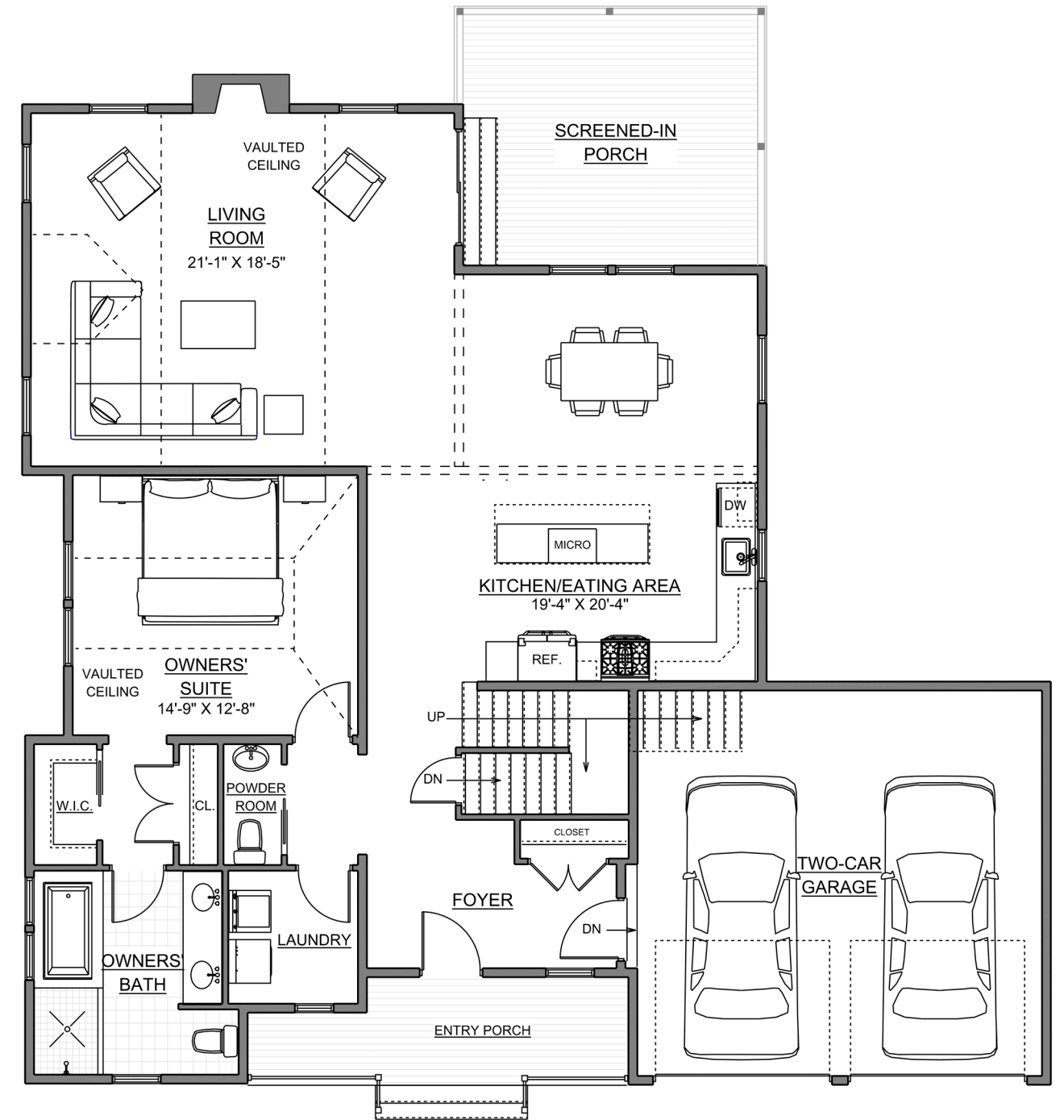
FIRST FLOOR PLAN - 1,523 G.S.F.
