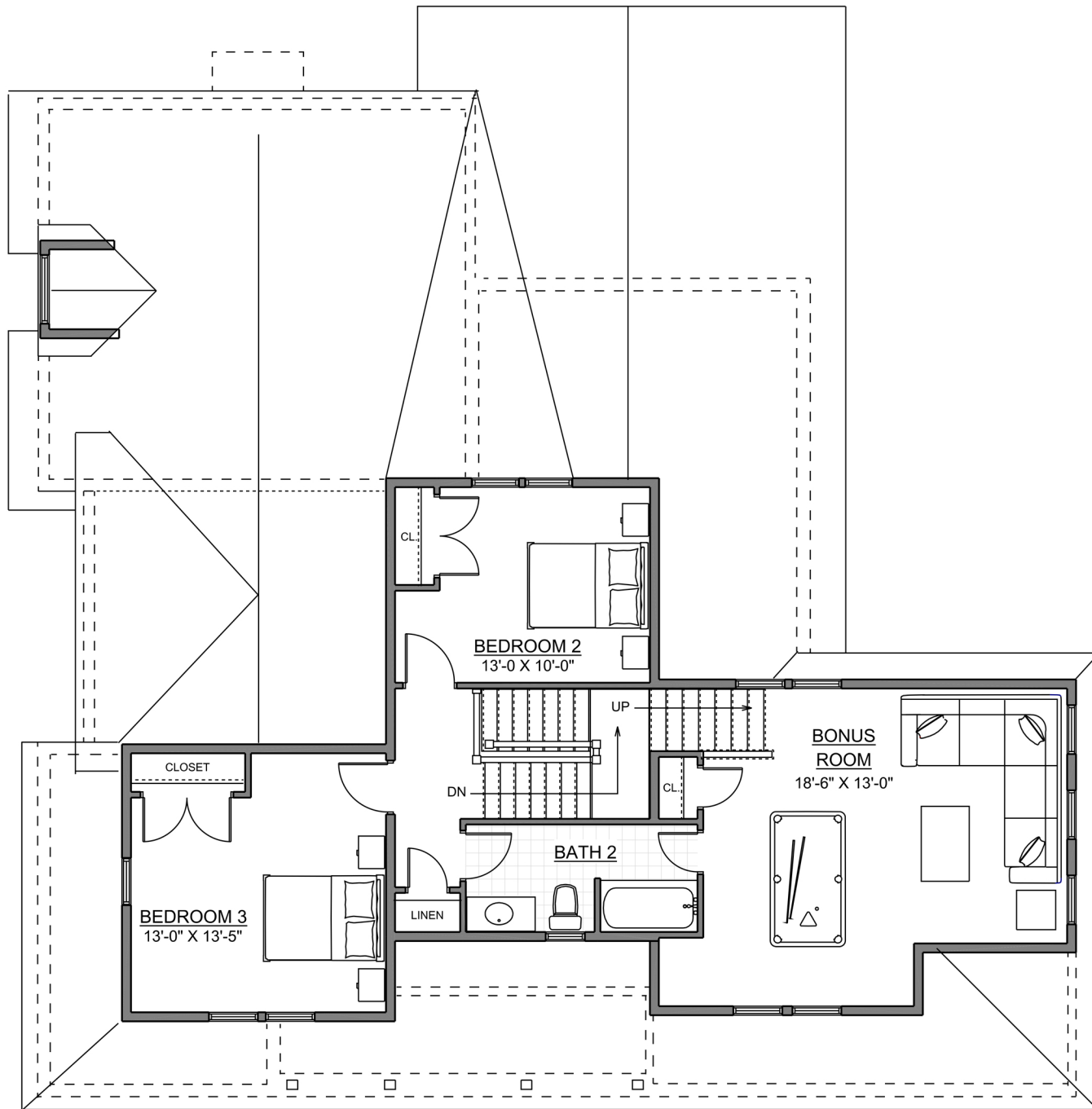
SECOND FLOOR PLAN - 826 G.S.F.
